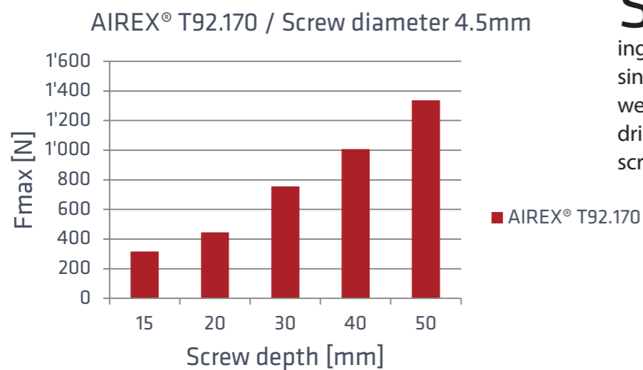
Fig. 3. Screw pull-out forces: depending on screw-in depth, screw type, and foam density, forces exceeding 1'000 N can be achieved.
