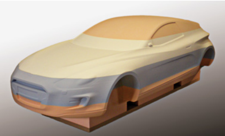
Automotive design model made of SikaBlock® ML range. The combination of superior surface quality and the use of dedicated adhesive SikaBiresin® B200 enables an easy painting without showing glue lines. Credit: Estech Design
