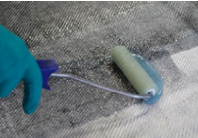
Wet lay-up with SikaBiresin CR168
